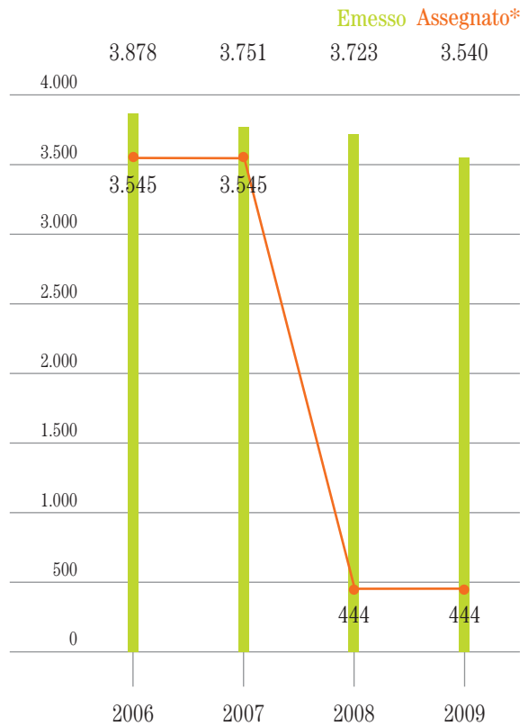
Emissioni CO 2 IGCC (ton/anno)
