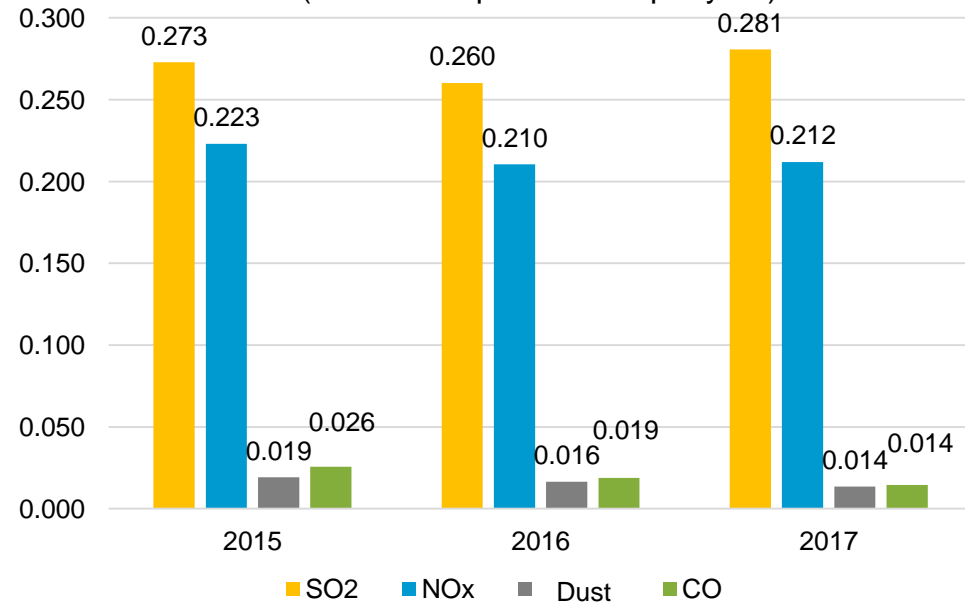
Conveyed emission index (t emitted/kt processed per year)
